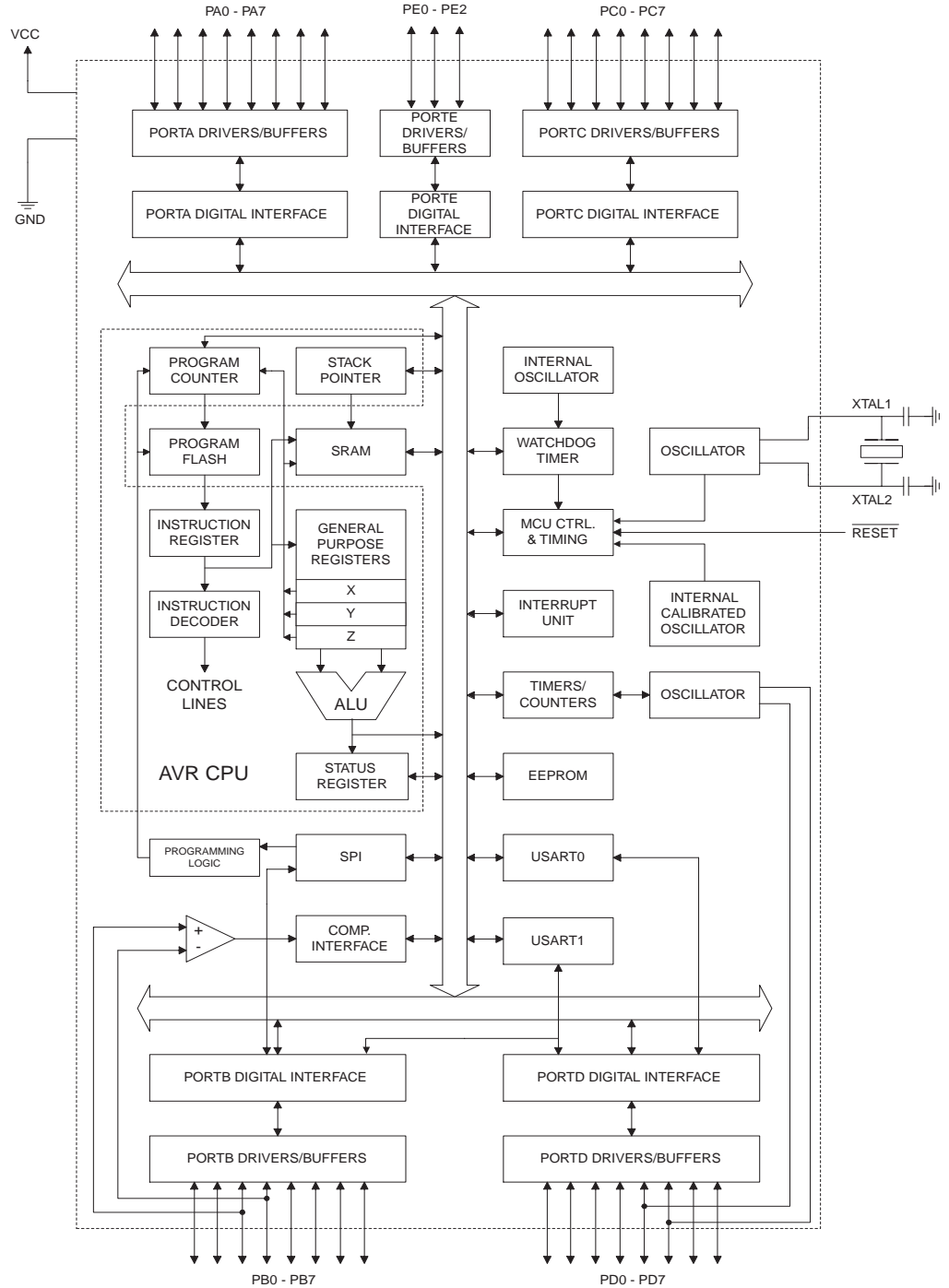
Figure 2. Block Diagram
